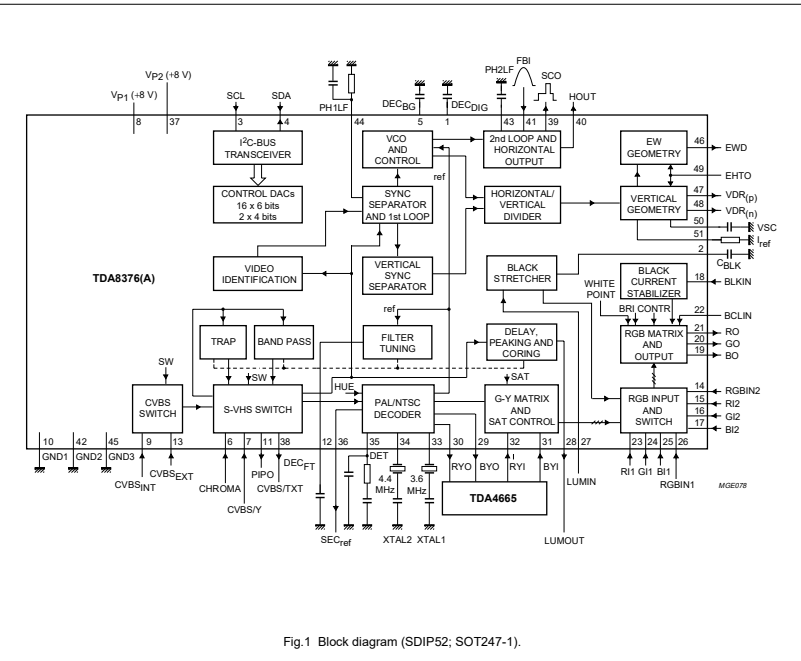
Fig.1 Block diagram (SDIP52; SOT247-1).
