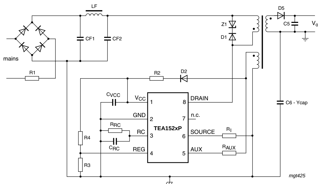
Fig 6. Primary sensed application; configuration for TEA152xP (DIP8)
