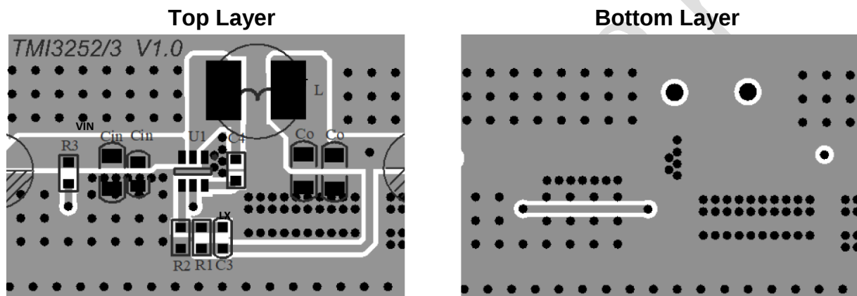
Figure 3. Sample of PCB Layout (TMI3252)
