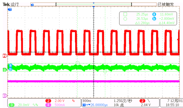
Iout=50% load
