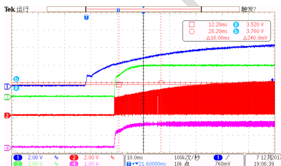
Power on , Iout= 1.2A
