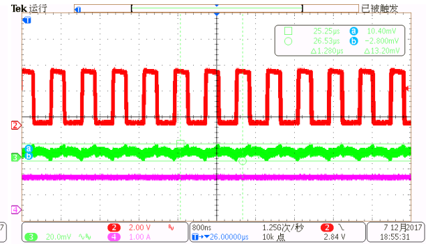
Iout=100% load
