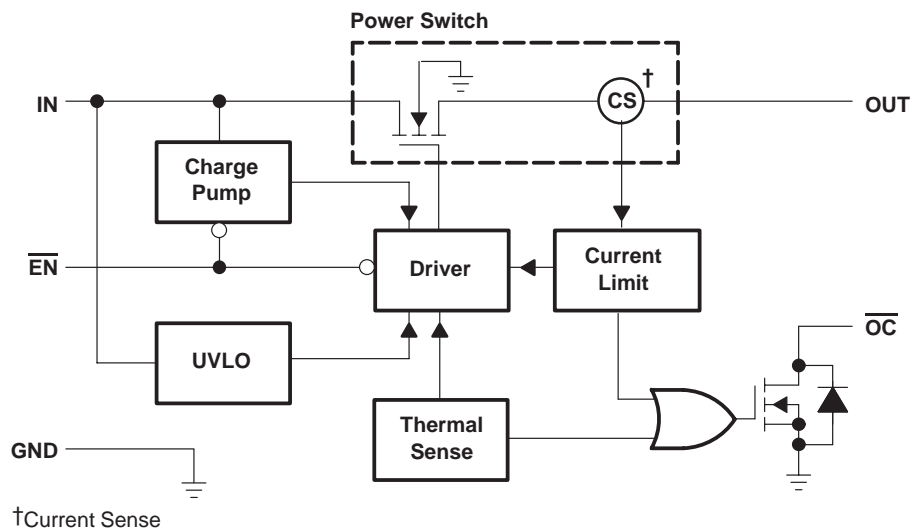
TPS2041 functional block diagram
