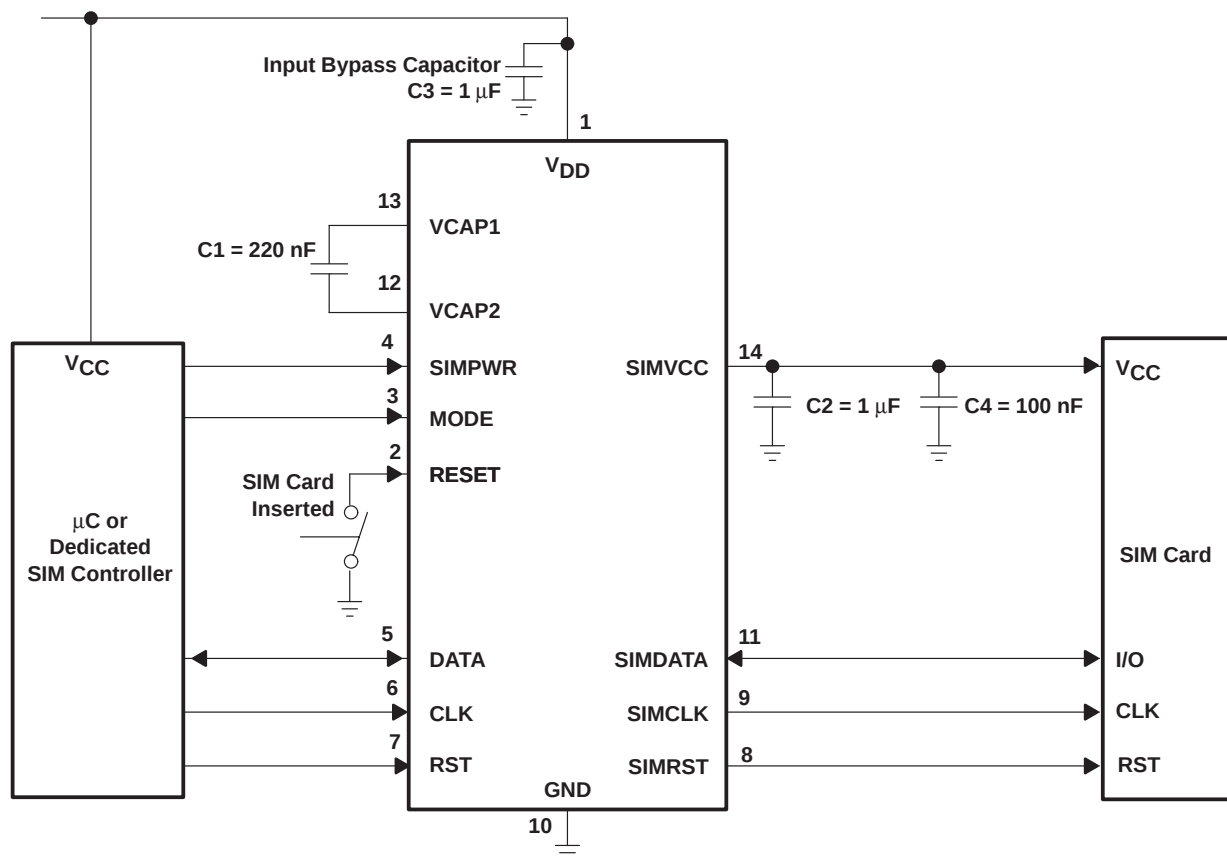
Figure 27. Typical Application
