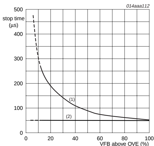
Fig 16. Shutdown time at over voltage extra detection
