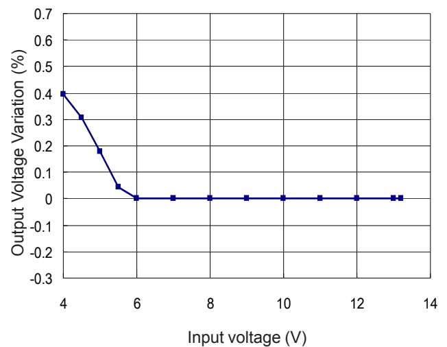
Line Regulation
