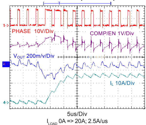
Load Transient Response Response
