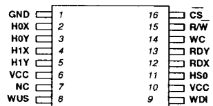
2-Channel 16-lead SOIC
