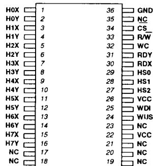
8-Channel 36-lead SOIC
