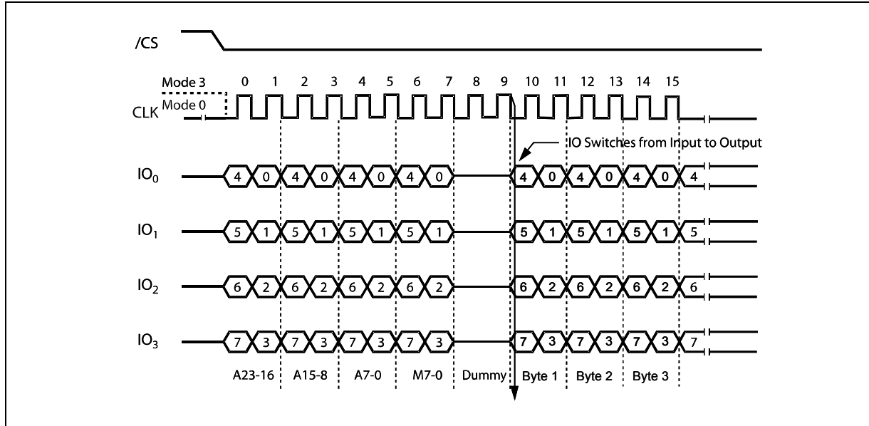
Figure 14b. Word Read Quad I/O Instruction Sequence Diagram (M7-0 = Axx)
