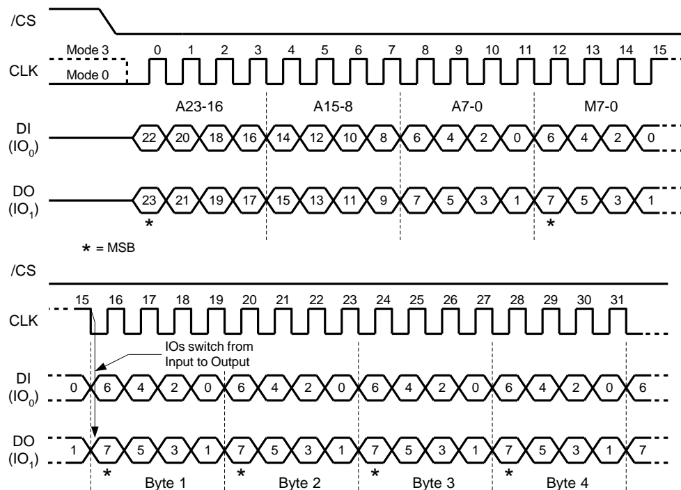
Figure 22b. Fast Read Dual I/O Instruction (Previous instruction set M5-4 = 10, SPI Mode only)
