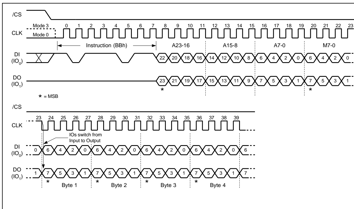
Figure 13a. Fast Read Dual I/O Instruction Sequence (Initial instruction or previous M5-4 \neq 10)
