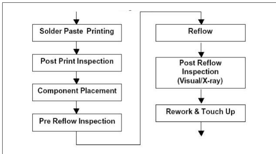
Figure 32. Assembly Flow
