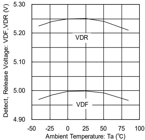
XC61X1~XC61X7 (5.0V)
