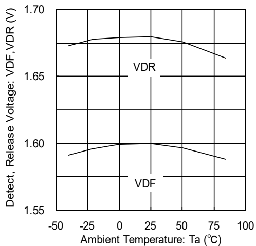
XC61X1~XC61X7 (1.6V)
